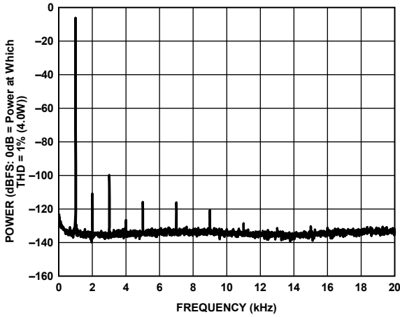
Figure 5. 1 W Output Power into 6 Ω Load, PVDD = 12 V
