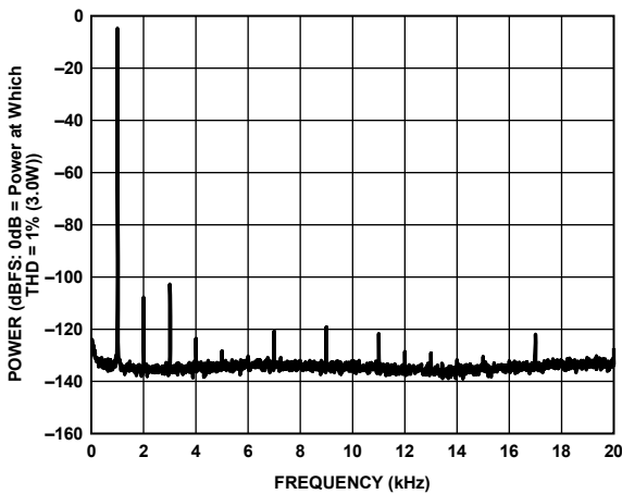
Figure 6. 1 W Output Power into 8 Ω Load, PVDD = 12 V
