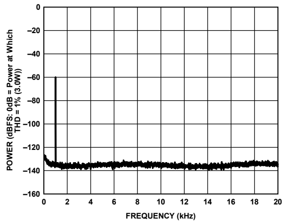
Figure 9. -60 dBFS Output Power into 8 Ω Load, PVDD = 12 V
