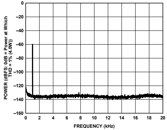
Figure 8. -60 dBFS Output Power into 6 Ω Load, PVDD = 12 V
