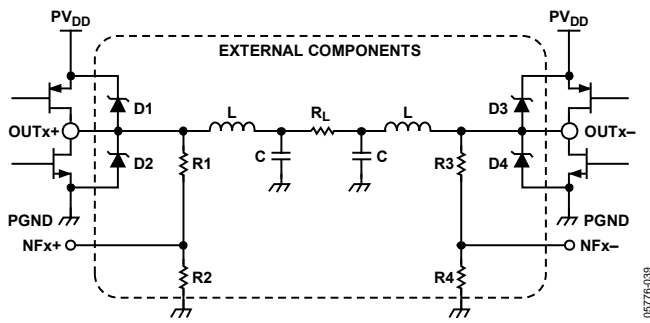
Figure 35. H-Bridge Configuration
