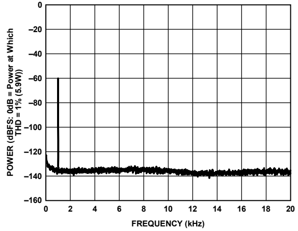
Figure 7. -60 dBFS Output Power into 4 Ω Load, PVDD = 12 V
