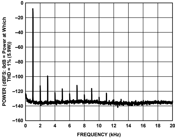
Figure 4. 1 W Output Power into 4 Ω Load, PVDD = 12 V
