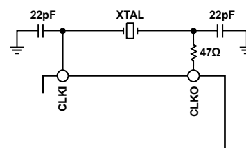
Figure 37. Crystal Connection
